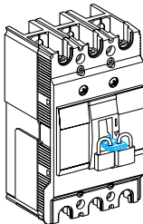
Toggle locking using a removable device: for EZC100/125
