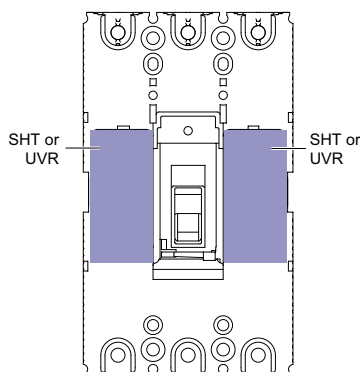
SHT and UVR releases on EZC100/125.
