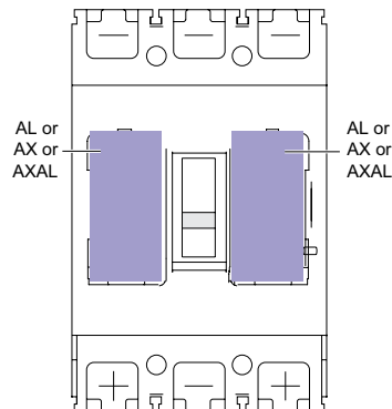
AXAL and AX electrical auxiliaries on EZC100/125
