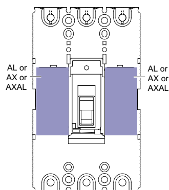
AXAL and AX electrical auxiliaries on EZC100/125
