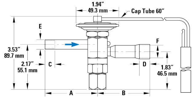
Bulb Sizes
