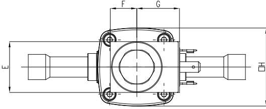
Solenoid valves with coil and connector - ODS
