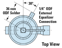
Dimensions - Connections
