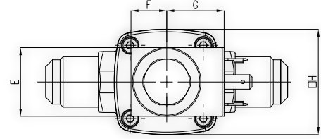
Solenoid valves with coil and connector - SAE Selenoid valfler Bobin ve konnektörlü - SAE
